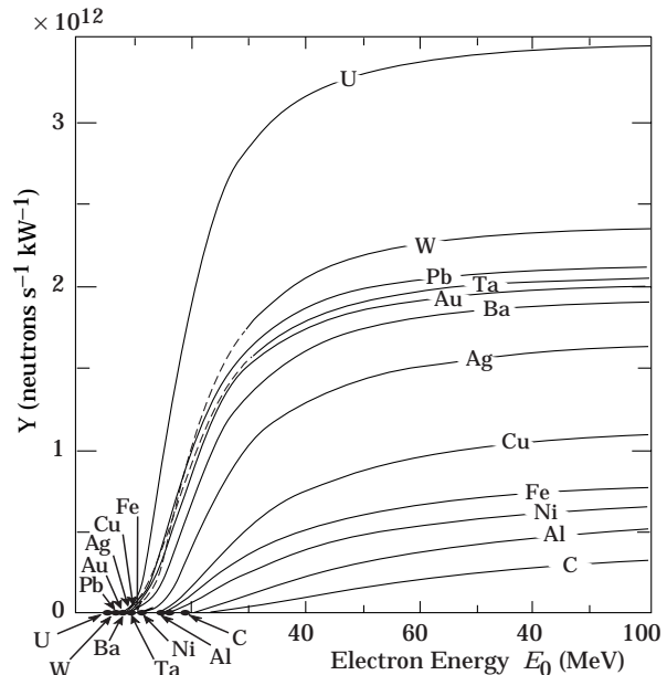
Figure 25.1: Neutron yields from semi-infinite targets, per kW of electron beam power, as a function of electron beam energy, disregarding target self-shielding.
