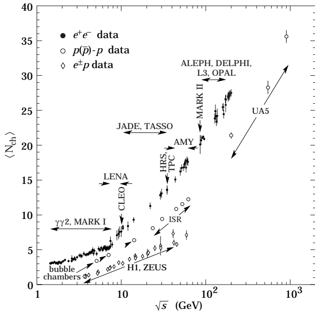
Figure 38.5: Average multiplicity as a function of \sqrt{s} for e^+e^- and p\bar{p} annihilations, and pp and ep collisions. The indicated errors are statistical and systematic errors added in quadrature, except when no systematic errors are given. Files of the data shown in this figure are given in http://home.cern.ch/b/biebel/www/RPP02
