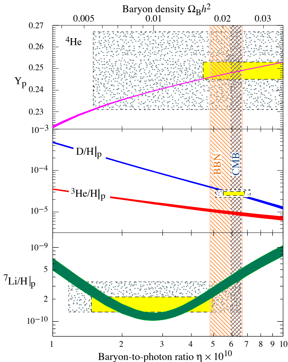
Figure 20.1: The abundances of {}^4\text{He} , D, {}^3\text{He} , and {}^7\text{Li} as predicted by the standard model of big-bang nucleosynthesis — the bands show the 95% CL range. Boxes indicate the observed light element abundances (smaller boxes: \pm 2\sigma statistical errors; larger boxes: \pm 2\sigma statistical and systematic errors). The narrow vertical band indicates the CMB measure of the cosmic baryon density, while the wider band indicates the BBN concordance range (both at 95% CL).
