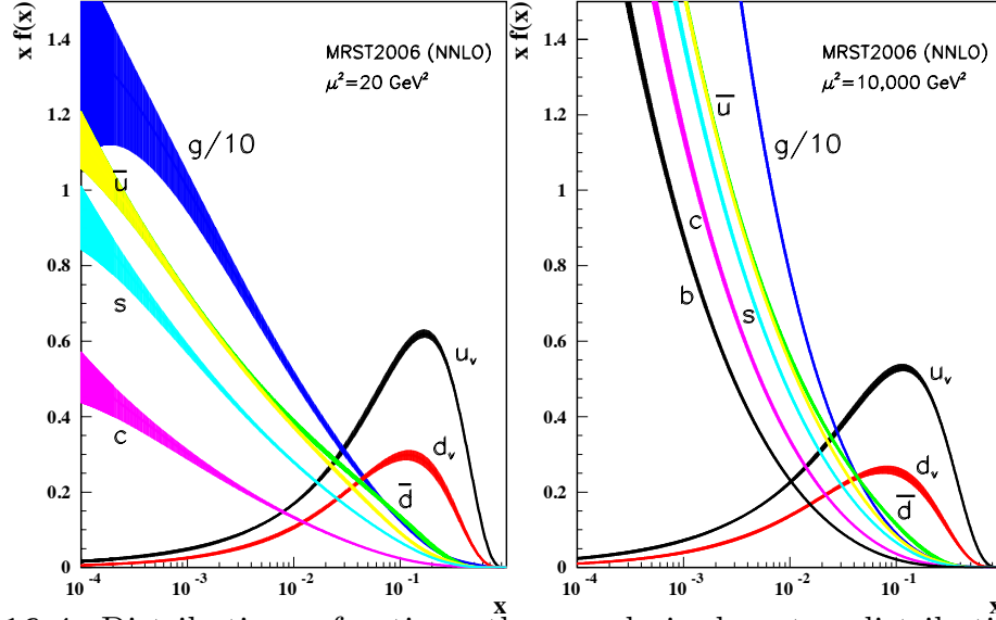
Figure 16.4: Distributions of x times the unpolarized parton distributions f(x) (where f = u_v, d_v, \bar{u}, \bar{d}, s, c, b, g ) and their associated uncertainties using the NNLO MRST2006 parameterization [13] at a scale \mu^2 = 20 \text{ GeV}^2 and \mu^2 = 10,000 \text{ GeV}^2 .
