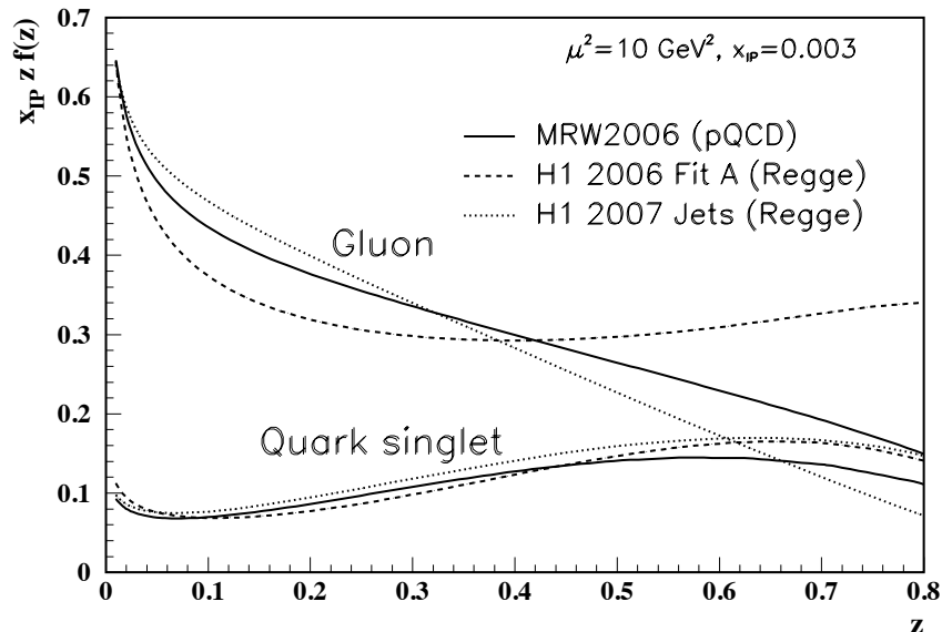
Figure 16.6: Diffractive parton distributions, x_{IP} z f_{a/p}^D , obtained from fitting to the H1 data with Q^2 > 8.5 \text{ GeV}^2 assuming Regge factorization [74], and using a more perturbative QCD approach [77]. Only the Pomeron contributions are shown and not the secondary Reggeon contributions which are negligible at the value of x_{IP} = 0.003 chosen here. Diffractive DIS dijet data [78,79,80] favour a smaller gluon at high z than that in H1 Fit A, more like MRW, as shown by the H1 Jets curve [79].
