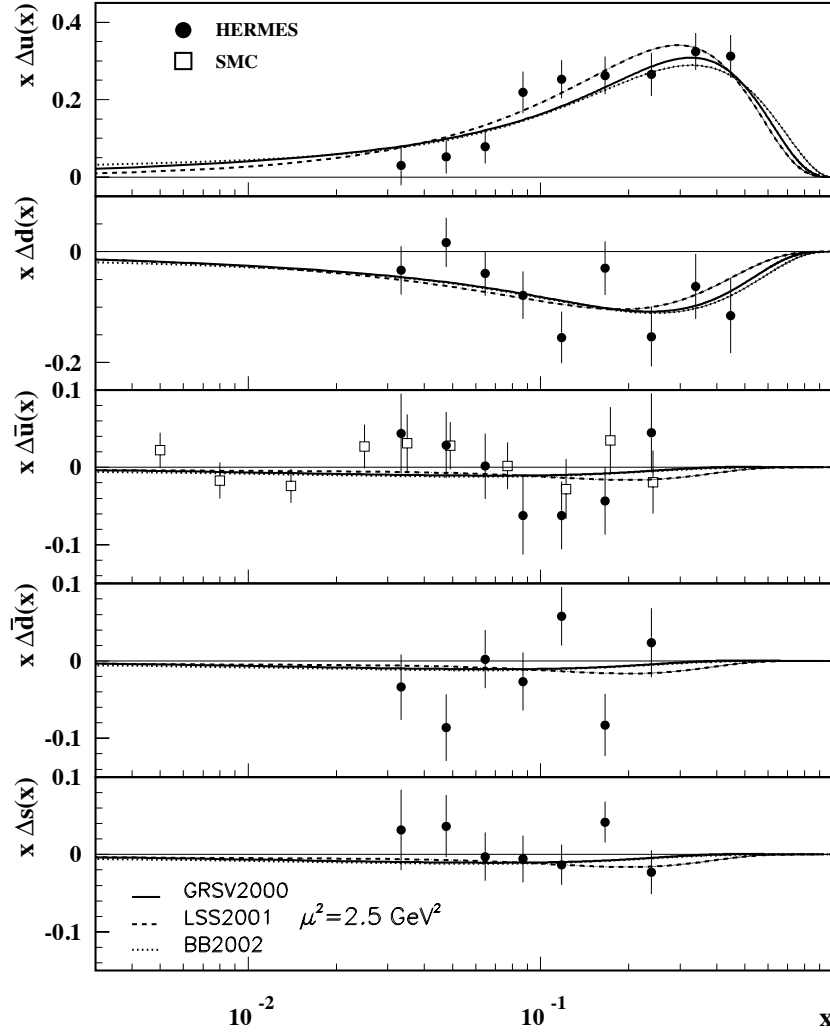
Figure 16.5: Distributions of x times the polarized parton distributions \Delta q(x) (where q = u, d, \bar{u}, \bar{d}, s ) using the GRSV2000 [50], LSS2001 [51], and BB2002 [52] parameterizations at a scale \mu^2 = 2.5 \text{ GeV}^2 . Points represent data from semi-inclusive positron (HERMES [53]) and muon (SMC [54]) deep inelastic scattering given at Q^2 = 2.5 \text{ GeV}^2 . SMC results are extracted under the assumption that \Delta \bar{u}(x) = \Delta \bar{d}(x) .
