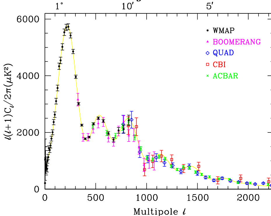
Figure 23.2: Band-power estimates from the WMAP , BOOMERANG , QUAD , CBI , and ACBAR experiments. Some of the low- \ell and high- \ell band-powers which have large error bars have been omitted. Note also that the widths of the \ell -bands varies between experiments and have not been plotted. This figure represent only a selection of available experimental results, with some other data-sets being of similar quality. The multipole axis here is linear, so the Sachs-Wolfe plateau is hard to see. However, the acoustic peaks and damping region are very clearly observed, with no need for a theoretical curve to guide the eye; the curve plotted is a best-fit model from WMAP 5-year plus other CMB data.
