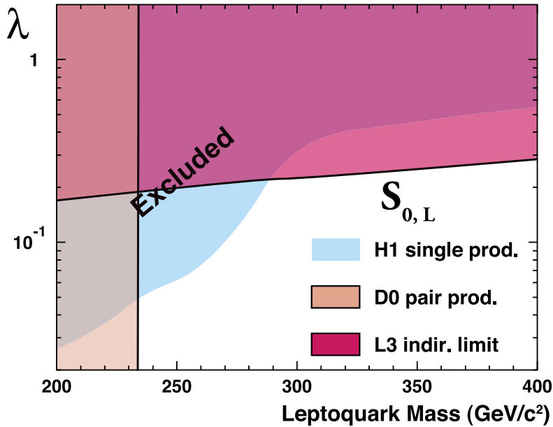
Figure 1: Limits on two typical first-generation scalar leptoquark states in the mass-coupling plane. The upper figure is for a weak-isodoublet, weak-hypercharge 7/6 , 3B + L = 0 leptoquark state, while the lower figure for a weak-isosinglet, weak-hypercharge -1/3 , 3B + L = 2 state. Color version at end of book.
