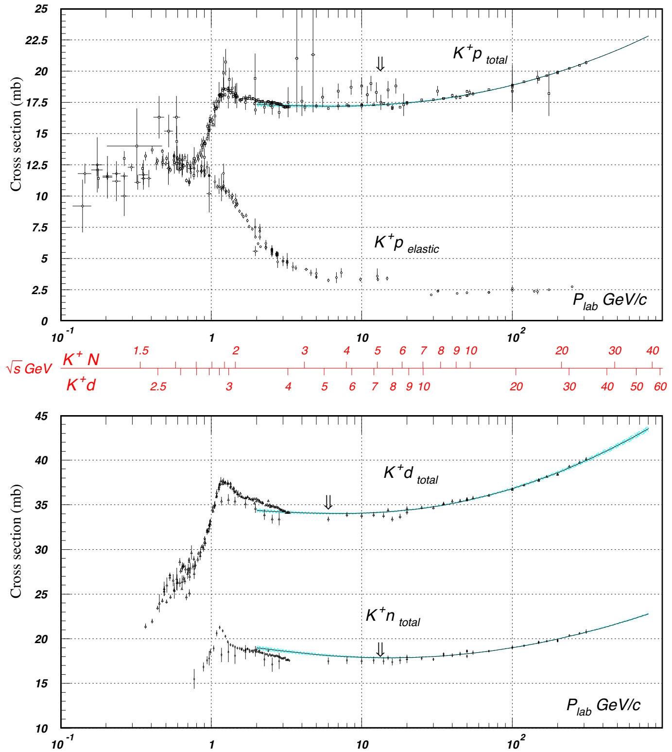
Figure 44.14: Total and elastic cross sections for K^+p and total cross sections for K^+d and K^+n collisions as a function of laboratory beam momentum and total center-of-mass energy. Corresponding computer-readable data files may be found at http://pdg.lbl.gov/current/xsect/ . (Courtesy of the COMPAS Group, IHEP, Protvino, April 2012)
