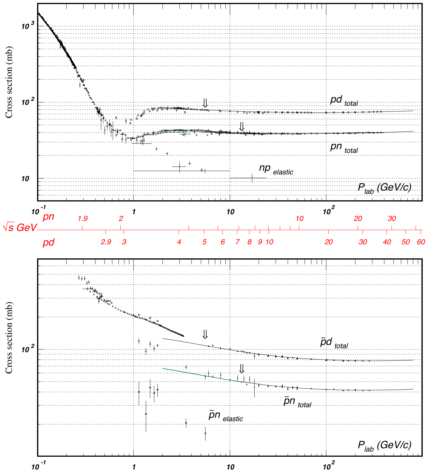
Figure 44.11: Total and elastic cross sections for pd (total only), np , p̄d (total only), and p̄n collisions as a function of laboratory beam momentum and total center-of-mass energy. Corresponding computer-readable data files may be found at http://pdg.lbl.gov/current/xsect/ . (Courtesy of the COMPAS Group, IHEP, Protvino, April 2012)
