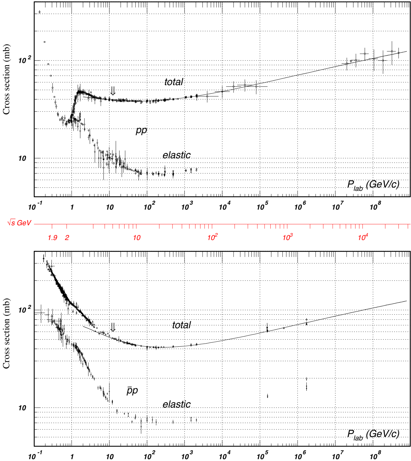
Figure 44.10: Total and elastic cross sections for pp and \bar{p}p collisions as a function of laboratory beam momentum and total center-of-mass energy. Corresponding computer-readable data files may be found at http://pdg.lbl.gov/current/xsect/ . (Courtesy of the COMPAS group, IHEP, Protvino, April 2012)
