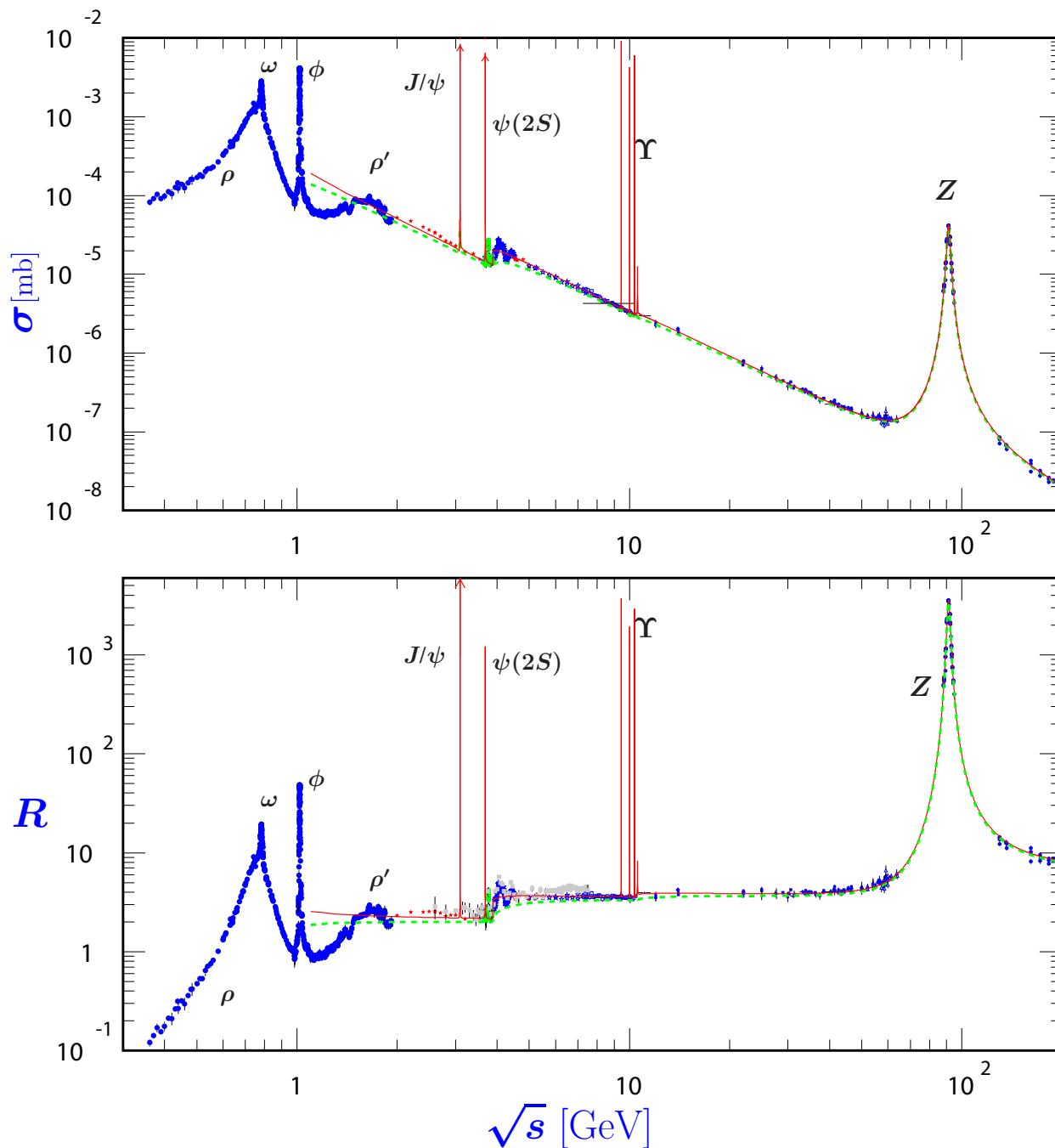
Figure 44.6: World data on the total cross section of e^+e^- \rightarrow \text{hadrons} and the ratio R(s) = \sigma(e^+e^- \rightarrow \text{hadrons}, s) / \sigma(e^+e^- \rightarrow \mu^+\mu^-, s) . \sigma(e^+e^- \rightarrow \text{hadrons}, s) is the experimental cross section corrected for initial state radiation and electron-positron vertex loops, \sigma(e^+e^- \rightarrow \mu^+\mu^-, s) = 4\pi\alpha^2(s)/3s . Data errors are total below 2 GeV and statistical above 2 GeV. The curves are an educative guide: the broken one (green) is a naive quark-parton model prediction, and the solid one (red) is 3-loop pQCD prediction (see “Quantum Chromodynamics” section of this Review, Eq. (9.7) or, for more details, K. G. Chetyrkin et al. , Nucl. Phys. B586 , 56 (2000) (Erratum ibid. B634 , 413 (2002))). Breit-Wigner parameterizations of J/\psi , \psi(2S) , and \Upsilon(nS) , n = 1, 2, 3, 4 are also shown. The full list of references to the original data and the details of the R ratio extraction from them can be found in [arXiv:hep-ph/0312114]. Corresponding computer-readable data files are available at http://pdg.lbl.gov/current/xsect/ . (Courtesy of the COMPAS (Protvino) and HEPDATA (Durham) Groups, May 2010.)
