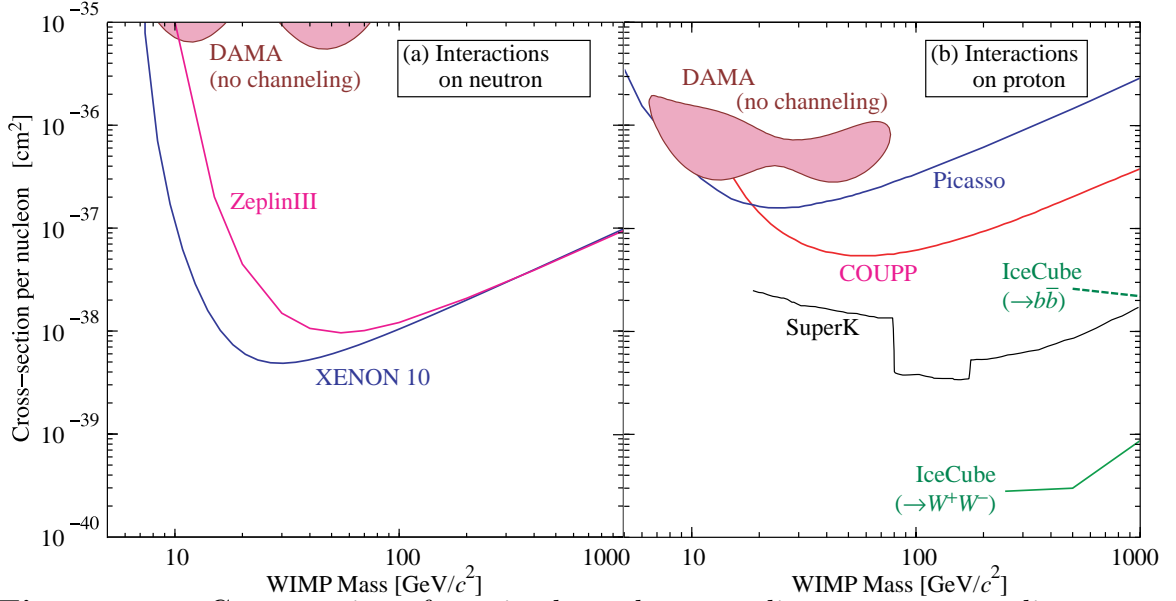
Figure 24.2: Cross sections for spin dependent coupling versus mass diagrams. References to the experimental results are given in the text. The DAMA candidates region (no channeling) are from [50]: (a) interactions on neutron; (b) interactions on proton.
