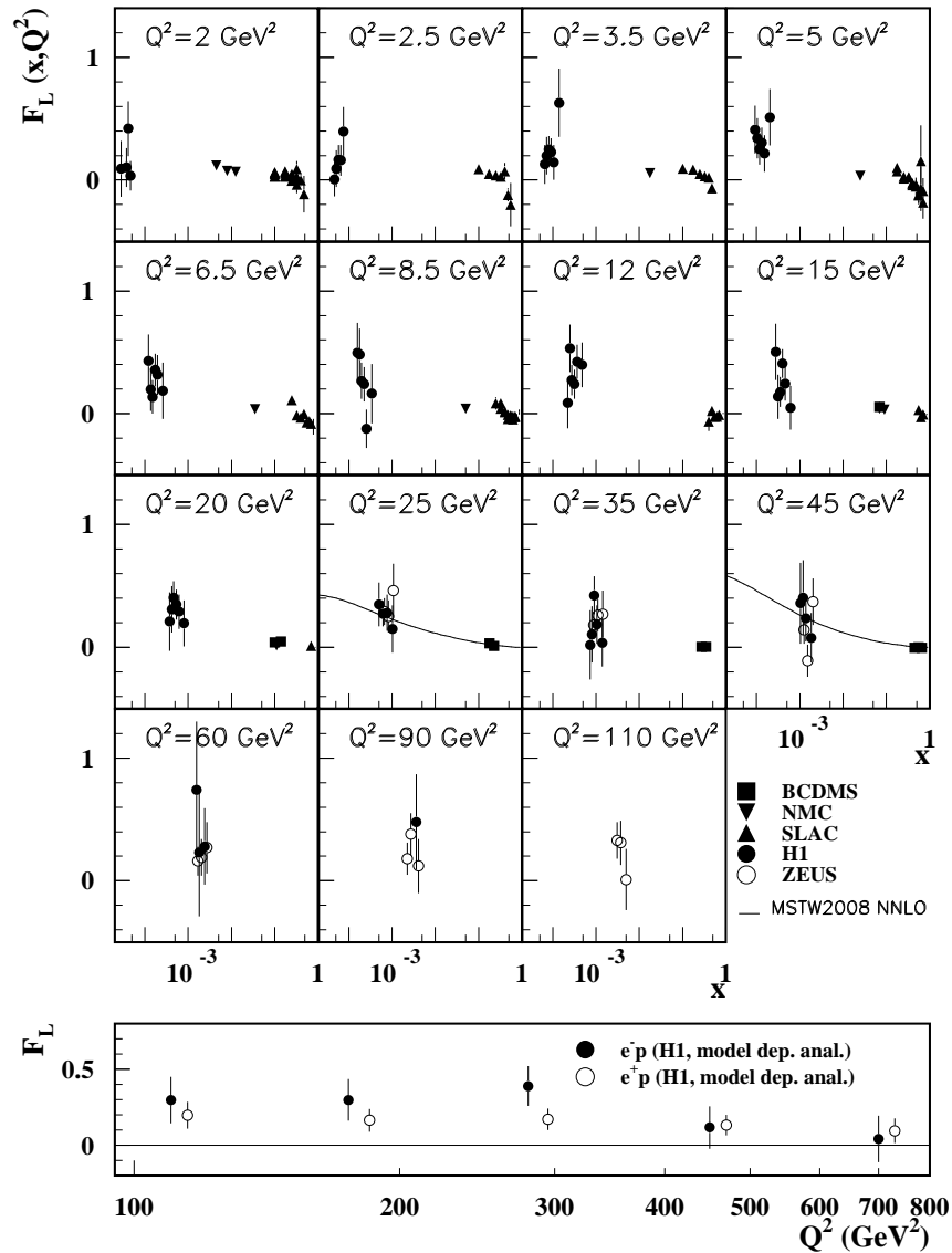
Figure 18.13: Top panel: The longitudinal structure function F_L as a function of x in bins of fixed Q^2 measured on the proton (except for the SLAC data which also contain deuterium data). BCDMS, NMC, and SLAC results are from measurements of R (the ratio of longitudinal to transverse photon absorption cross sections) which are converted to F_L by using the BCDMS parameterization of F_2 (A.C. Benvenuti et al. , Phys. Lett. B223 , 485 (1989)). It is assumed that the Q^2 dependence of the fixed-target data is small within a given Q^2 bin. Some of the other data may have been rebinned to common Q^2 values. Also shown is the MSTW2008 parameterization given at two Q^2 values (A.D. Martin et al. , Eur. Phys. J. C63 , 189 (2009)). References: H1 —F.D. Aaron et al. , Phys. Lett. B665 , 139 (2008); F.D. Aaron et al. , Eur. Phys. J. C71 , 1579 (2011); ZEUS —S. Chekanov et al. , Phys. Lett. B682 , 8 (2009); BCDMS —A. Benvenuti et al. , Phys. Lett. B223 , 485 (1989); NMC —M. Arneodo et al. , Nucl. Phys. B483 , 3 (1997); SLAC —L.W. Whitlow et al. , Phys. Lett. B250 , 193 (1990) and numerical values from the thesis of L.W. Whitlow (SLAC-357).
