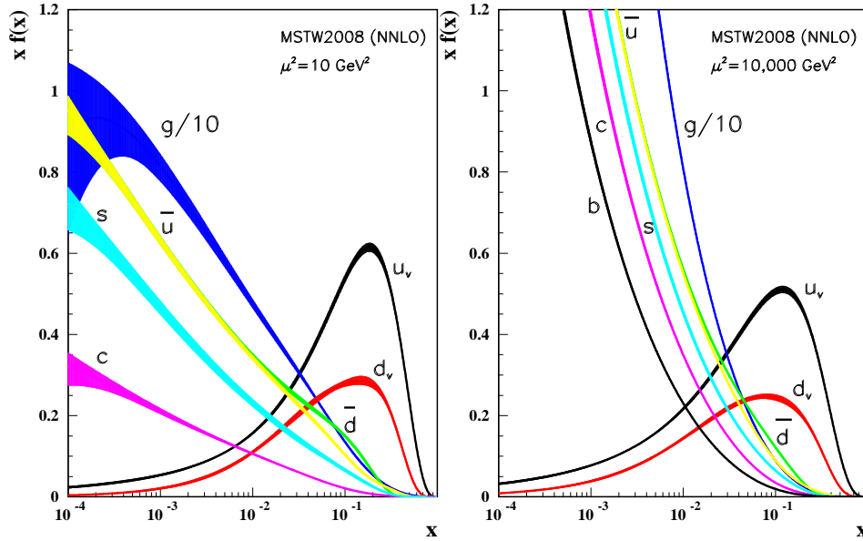
Figure 18.4: Distributions of x times the unpolarized parton distributions f(x) (where f = u_v, d_v, \bar{u}, \bar{d}, s, c, b, g ) and their associated uncertainties using the NNLO MSTW2008 parameterization [13] at a scale \mu^2 = 10 \text{ GeV}^2 and \mu^2 = 10,000 \text{ GeV}^2 .
