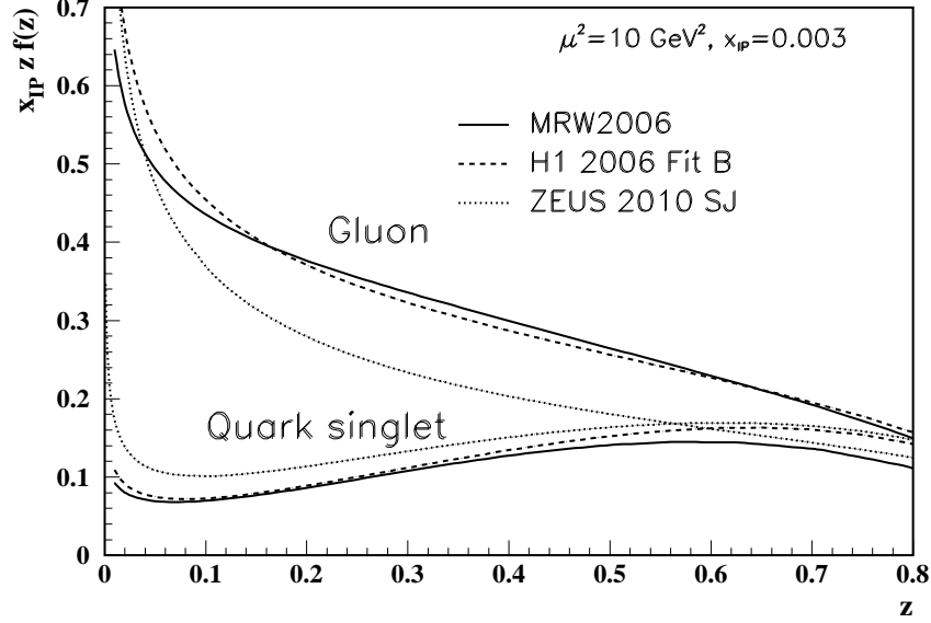
Figure 18.6: Diffractive parton distributions, x_{\mathbb{P}} z f_{a/p}^{\mathbb{D}} , obtained from fitting to the ZEUS data with Q^2 > 5 \text{ GeV}^2 [86], H1 data with Q^2 > 8.5 \text{ GeV}^2 assuming Regge factorization [81], and using a more perturbative QCD approach [87]. Only the Pomeron contributions are shown and not the secondary Reggeon contributions, which are negligible at the value of x_{\mathbb{P}} = 0.003 chosen here. The H1 2007 Jets distribution [88] is similar to H1 2006 Fit B.
