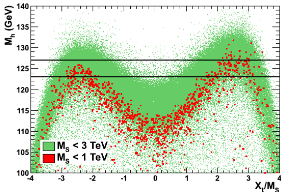
Figure 23: The maximal value of m_h as a function of X_t/M_{\text{SUSY}} ( M_{\text{SUSY}} \equiv M_S ) in the pMSSM when all other soft SUSY-breaking parameters and \tan\beta are scanned as defined in Ref. [253].
