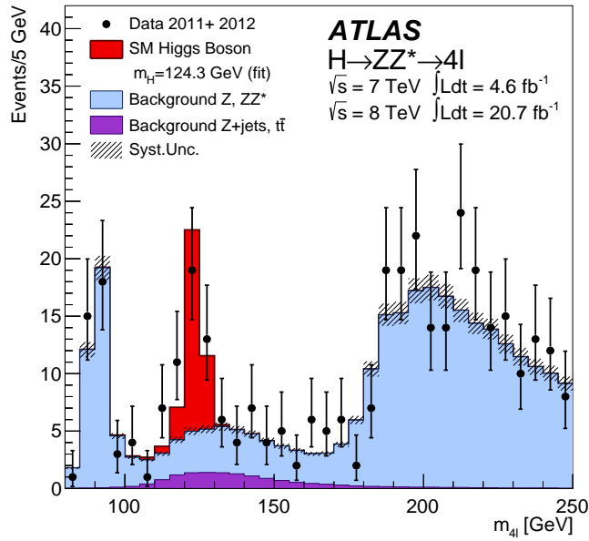
Figure 8: The combined m_{4\ell} distribution from ATLAS [119].
