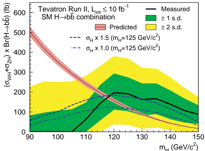
Figure 14: The combined CDF and D0 results on the best-fit cross section times branching ratio (\sigma_{WH} + \sigma_{ZH}) \times B(H \rightarrow b\bar{b}) as well as the SM prediction as a function of m_H [108].
