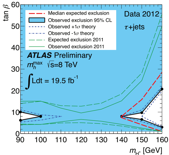
Figure 32: ATLAS exclusion limits of the searches of the light H^\pm , in the context of the MSSM m_h^{\max} scenario with \mu = 200 GeV [453]. For comparison, the 2011 limits are also indicated.
