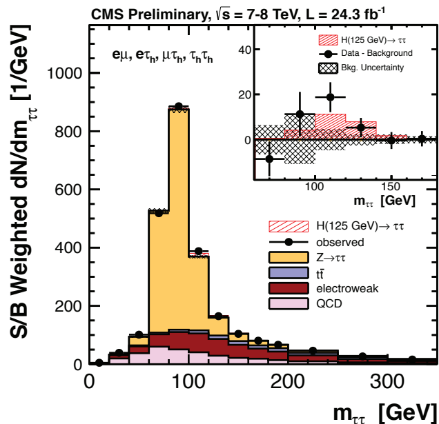
Figure 13: CMS results : The combined observed and expected m_{\tau\tau} distributions for all sub-channels combined. The insert shows the difference between the observed data and the expected background distributions, together with the expected signal distribution for a SM Higgs signal at m_H = 125 GeV [131].
