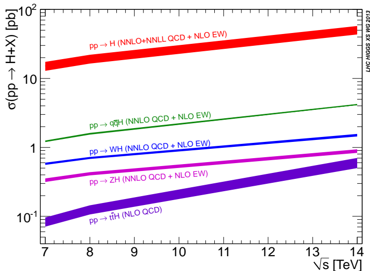
Figure 3: The SM Higgs boson production cross sections as a function of the center of mass energy, \sqrt{s} , for pp collisions. The theoretical uncertainties [39] are indicated as a band.
