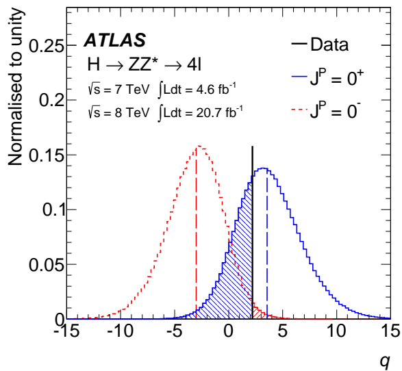
Figure 22: Expected distributions of q , for the Standard Model 0^+ (blue/solid line distribution) or 0^- (red/dashed line distribution) signals [197]. The observed value is indicated by the vertical solid line and the expected medians by the dashed lines. The colored areas correspond to the integrals of the expected distributions up to the observed value and are used to compute the p_0 -values for the rejection of each hypothesis.
