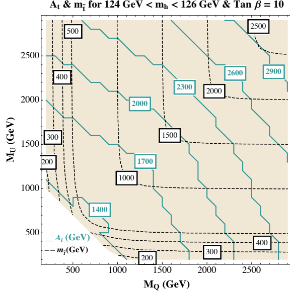
Figure 25: Contours of the stop mixing parameter, A_t , necessary for m_h to be in the 124–126 GeV range, given in the plane of the left- and right-handed stop soft supersymmetry-breaking mass parameters, M_Q and M_U , respectively. Other relevant parameters are fixed to be: \mu = 650 GeV, m_A = 1500 GeV, A_\tau = 500 GeV and \tan\beta = 10 . From Ref. [247].
