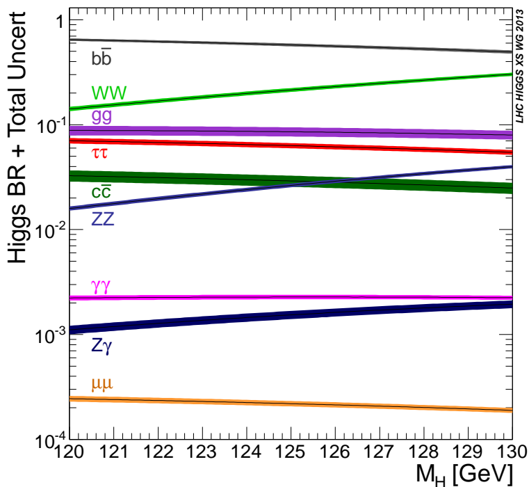
Figure 4: The branching ratios for the main decays of the SM Higgs boson near m_H = 125 GeV. The theoretical uncertainties [38] are indicated as a band.
