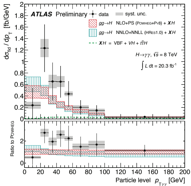
Figure 20: Observed differential cross sections in transverse momentum of the H in the diphoton channel, compared to the prediction of the ggH process [188].
