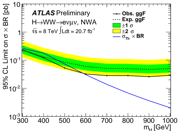
Figure 29: The 95% CL upper limits on the Higgs boson production cross section times branching ratio for H \rightarrow W^{(*)}W^{(*)} \rightarrow \ell\nu\ell\nu for the gluon-fusion process and a Higgs boson with a narrow lineshape (NWA). The green and yellow bands show the 1\sigma and 2\sigma uncertainties on the expected limit [478]. The expected cross section times branching ratio for the production of a SM Higgs boson is shown as a blue line.
