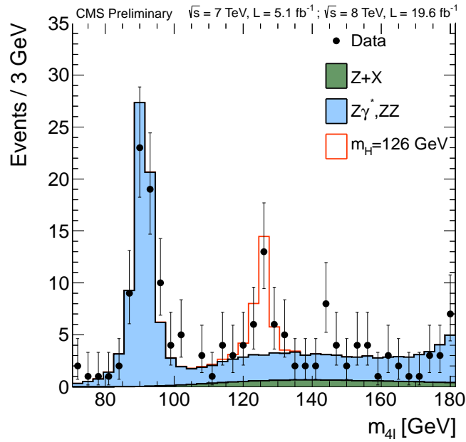
Figure 9: The combined m_{4\ell} distribution from CMS [121].
