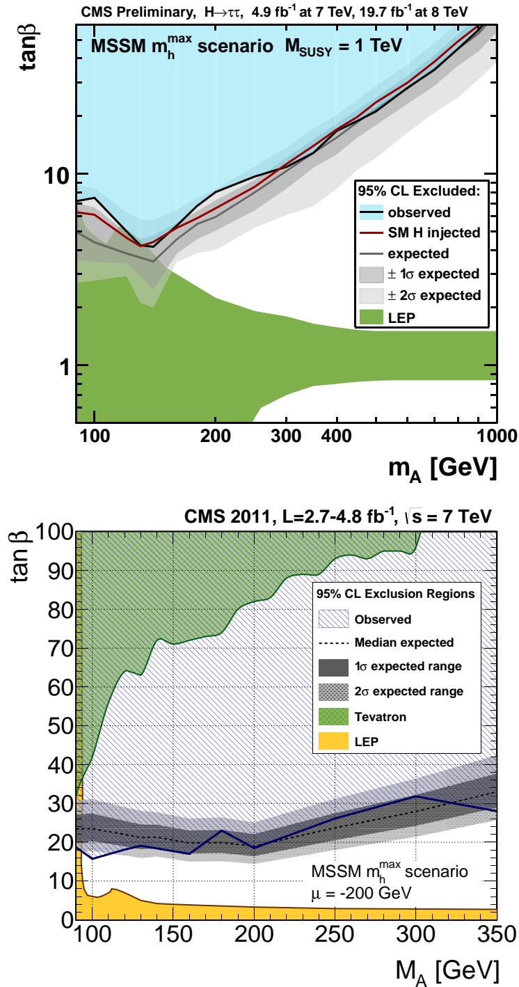
Figure 31: The 95% CL exclusion contours in the (M_A, \tan\beta) parameter space for the MSSM m_h^{\max} scenario, for the \tau^+\tau^- channel [446] (upper plot) and the b\bar{b} channel [448] (lower plot).
