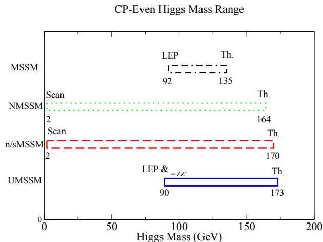
Figure 27: Mass ranges for the lightest CP -even Higgs boson in each extended MSSM scenario discussed in the text, and in the MSSM, for comparison. The value of M_{\text{SUSY}} is fixed to 1 TeV and the rest of parameters are scanned as defined in Ref. [343]. The radiative corrections are computed only at one loop level.
