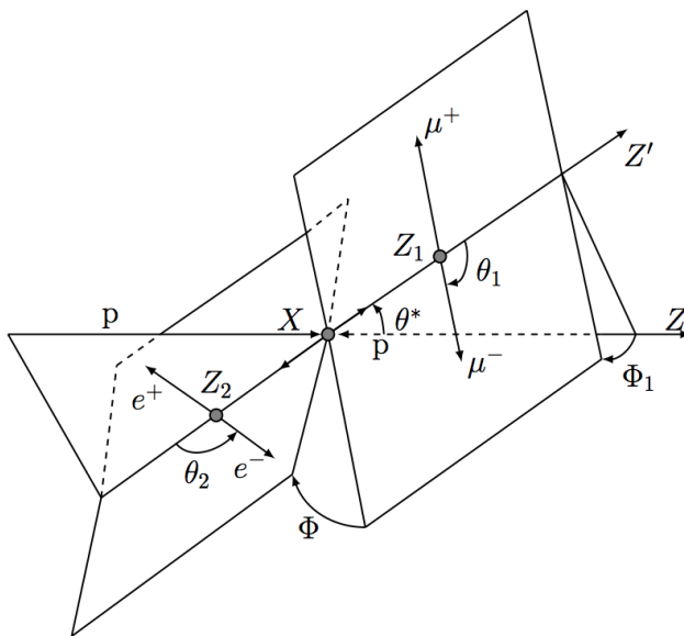
Figure 21: Definition of the production and decay angles defined for the H \rightarrow Z^{(*)}Z^{(*)} \rightarrow 4\ell final state [199].
