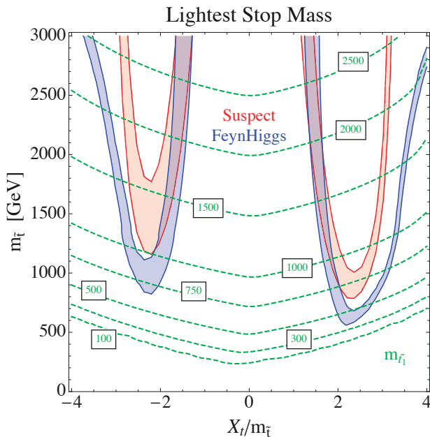
Figure 24: Contours of m_h in the MSSM as a function of m_{\tilde{t}} , a common stop mass M_Q = M_U , and the stop mixing parameter X_t for \tan\beta = 20 . The red/blue bands show the result from Suspect/FeynHiggs for m_h in the range 124–126 GeV. The contours of constant lightest stop mass are shown in green Ref. [254].
