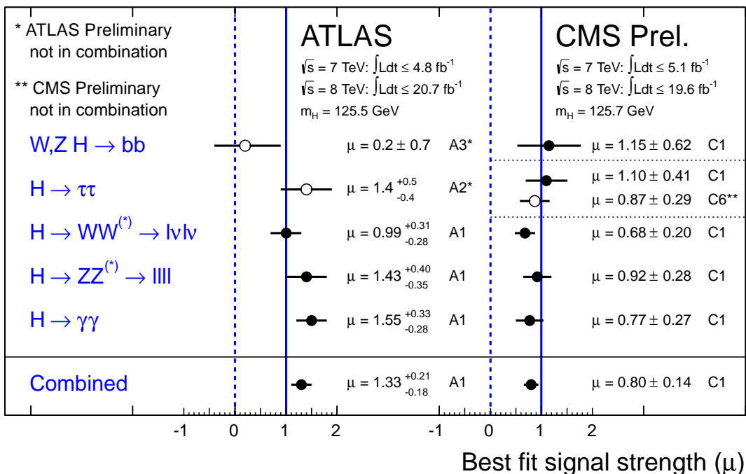
Figure 16: The signal strengths \mu measured by the ATLAS experiment from Refs. A1 [119], A2 [133] and A3 [138], and CMS experiment from Ref. C1 [124] and C6 [132] in the five principal channels and their combination. It should be noted that the ATLAS combination only includes the bosonic \gamma\gamma , ZZ and WW channels.
