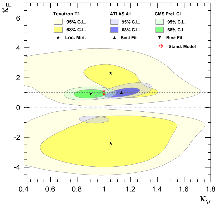
Figure 18: Likelihood contours of the global fit in the (\kappa_F, \kappa_V) plane for the ATLAS A1 [119], the CMS C1 [120] and the D0 and CDF combined T1 [108] results.
