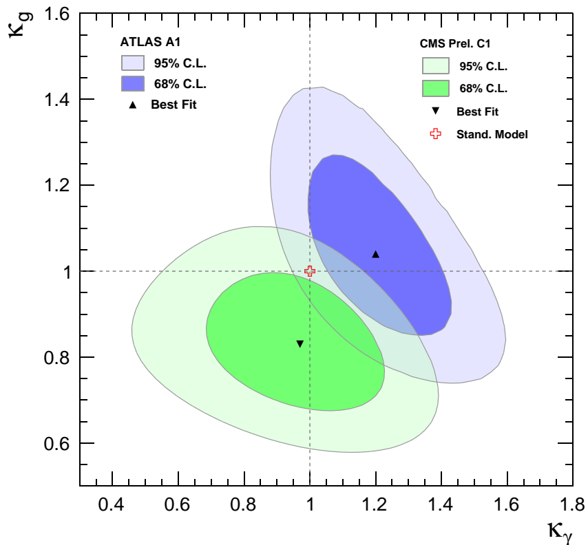
Figure 19: Likelihood contours of the global fit in the (\kappa_g, \kappa_\gamma) plane for the ATLAS experiment A1 [119] and the CMS experiment C1 [120] results.
