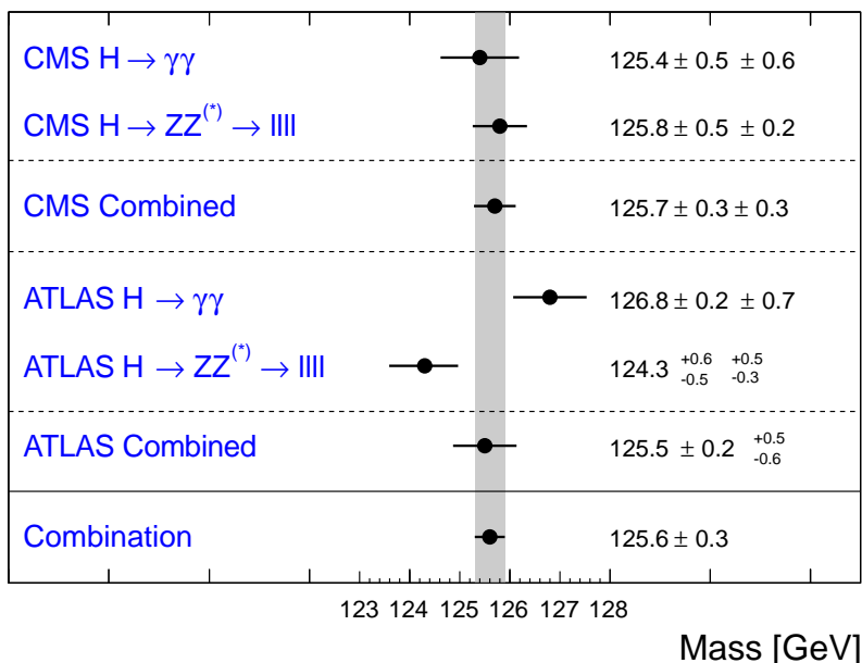
Figure 10: A compilation of the CMS and ATLAS mass measurements in the \gamma\gamma and ZZ channels, the combined result from each experiment and our average of the combinations.
