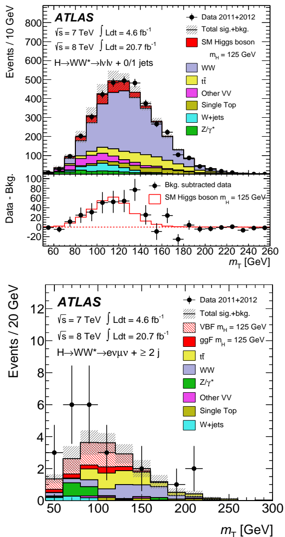
Figure 11: (Top) The m_T distribution for selected events summed over all lepton flavors and with \leq 1 associated jets. The observed excess over the estimated SM background and the expectation from a SM Higgs boson with m_H = 125 GeV are shown in the lower panel. (Bottom) The m_T distribution for selected e^\pm\mu^\mp events and with \geq 2 associated jets [119].
