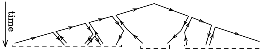
Figure 39.1: Color development of a shower in e^+e^- annihilation. Systems of color-connected partons are indicated by the dashed lines.
