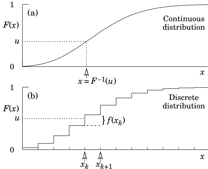
Figure 38.1: Use of a random number u chosen from a uniform distribution (0,1) to find a random number x from a distribution with cumulative distribution function F(x) .
