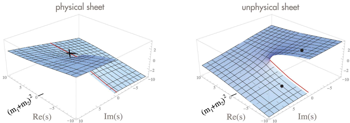
Figure 46.1: Sketch of the imaginary part of a typical single-channel amplitude in the complex s -plane. The solid dots indicate allowed positions for resonance poles, the cross for a bound state. The solid line is the physical axis (shifted by i\epsilon into the physical sheet). The two sheets are connected smoothly along their discontinuities.
