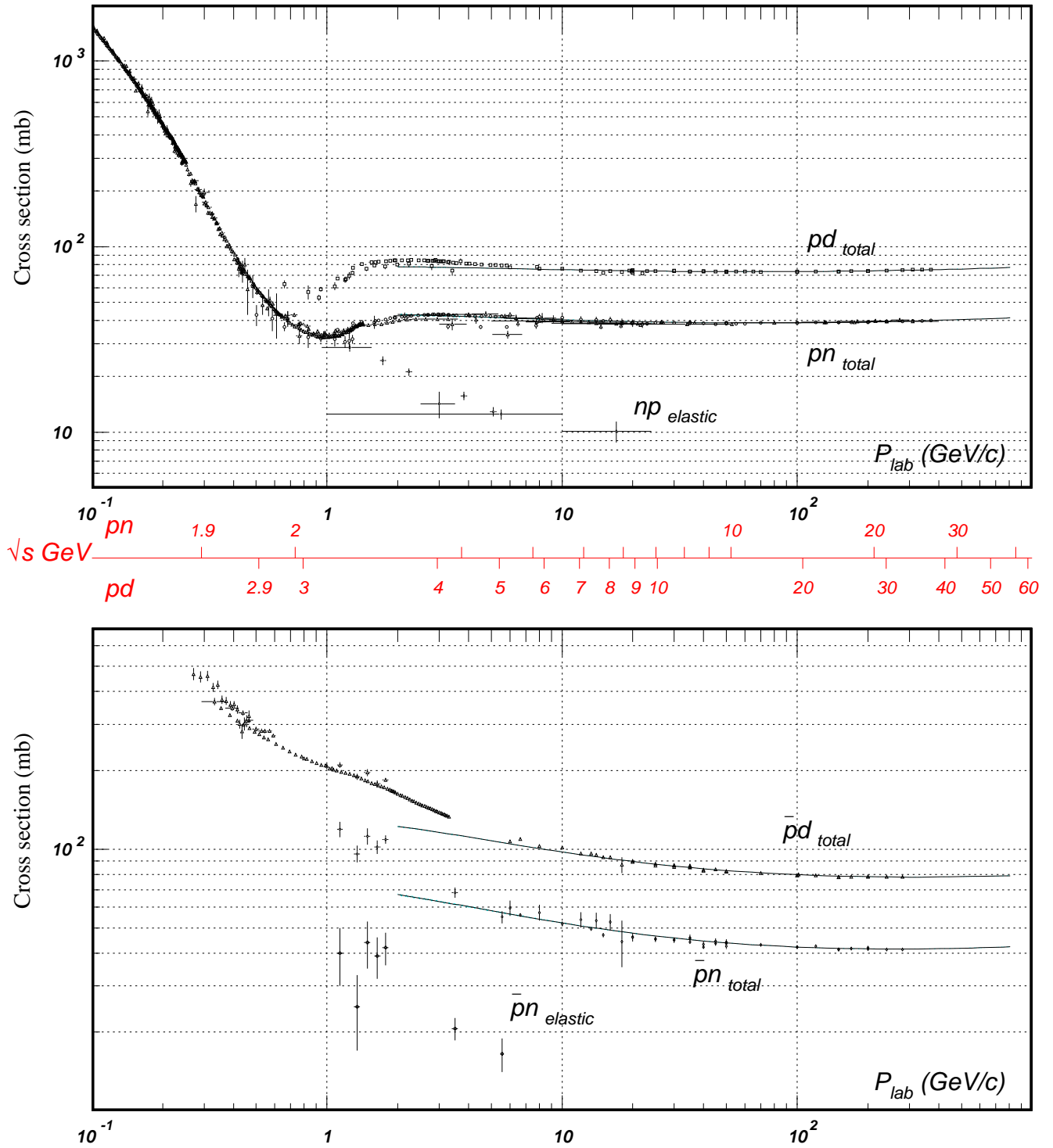
Figure 49.9D12: Total and elastic cross sections for pd (total only), np , \bar{p}d (total only), and \bar{p}n collisions as a function of laboratory beam momentum and total center-of-mass energy. Corresponding data files may be found at http://pdg.lbl.gov/xsect/contents.html (Courtesy of the COMPAS Group, IHEP, Protvino, September 2013.)
