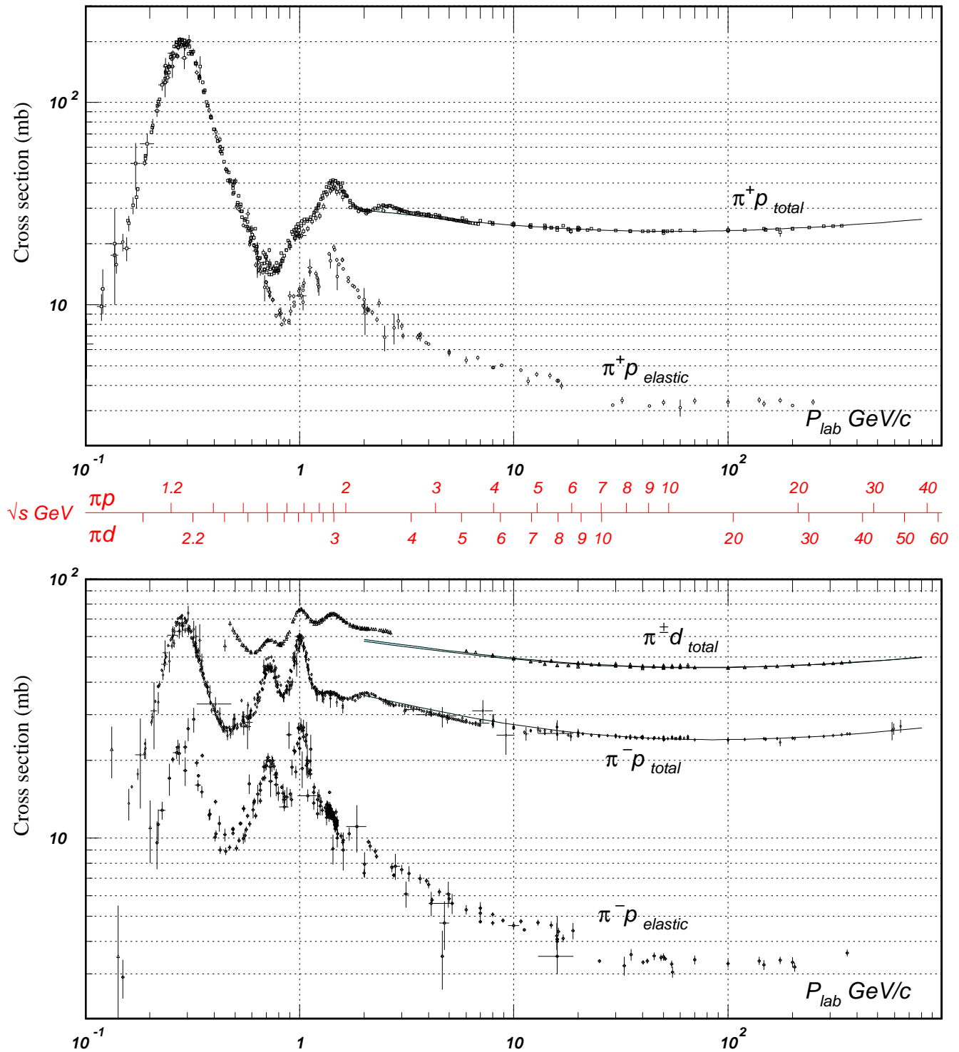
Figure 49.9D13: Total and elastic cross sections for \pi^\pm p and \pi^\pm d (total only) collisions as a function of laboratory beam momentum and total center-of-mass energy. Corresponding data files may be found at http://pdg.lbl.gov/xsect/contents.html (Courtesy of the COMPAS Group, IHEP, Protvino, September 2013.)
