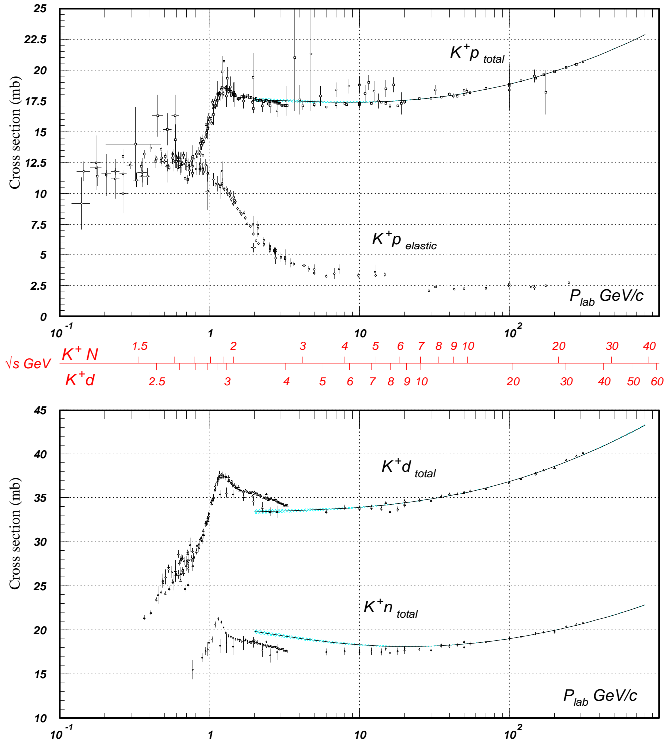
Figure 49.9D15: Total and elastic cross sections for K^+p and total cross sections for K^+d and K^+n collisions as a function of laboratory beam momentum and total center-of-mass energy. Corresponding data files may be found at http://pdg.lbl.gov/xsect/contents.html (Courtesy of the COMPAS Group, IHEP, Protvino, September 2013.)
