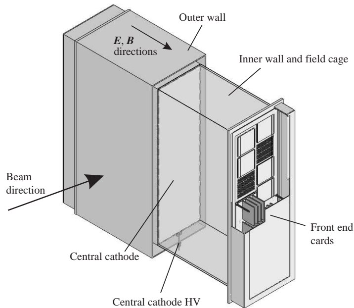
Figure 33.14: One of the 3 TPC modules for the near detector of the T2K experiment [107]. The size is 2 \times 2 \times 0.8 \text{ m}^3 . Micromegas devices are used for gas amplification and readout.
