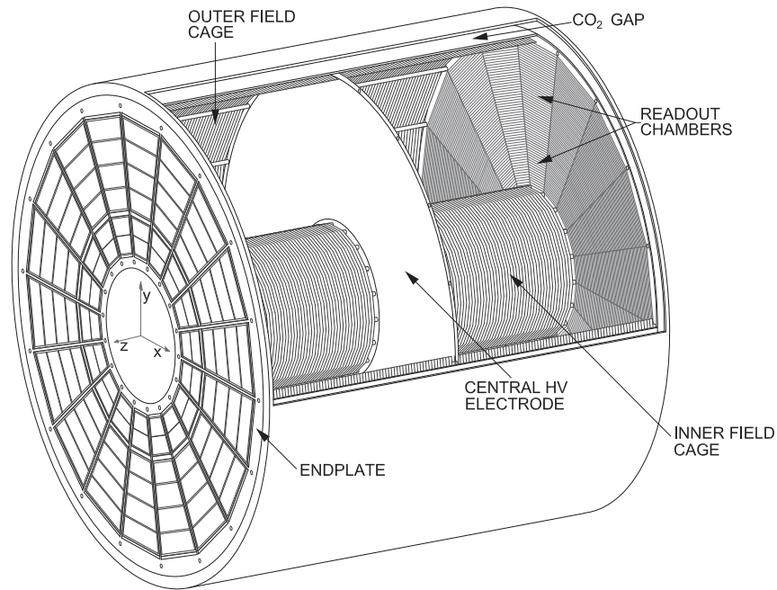
Figure 33.13: Schematic view of the ALICE TPC [106]. The drift volume with 5 m diameter is divided into two halves, each providing 2.5 m drift length.
