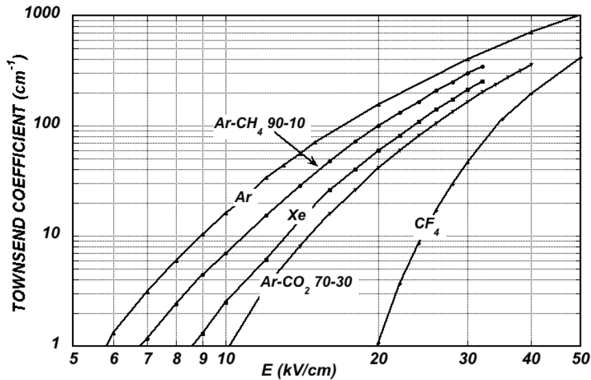
Figure 33.6: Computed first Townsend coefficient \alpha as a function of electric field in several gases at NTP [71].
