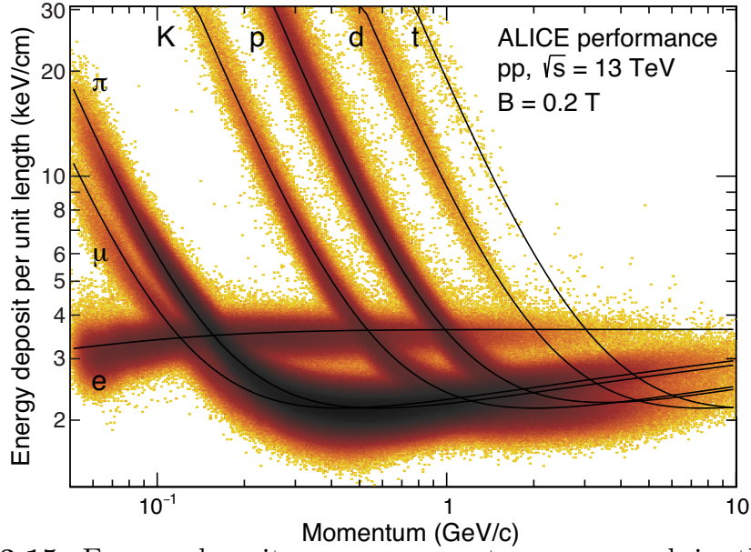
Figure 33.15: Energy deposit versus momentum measured in the ALICE TPC [108].
