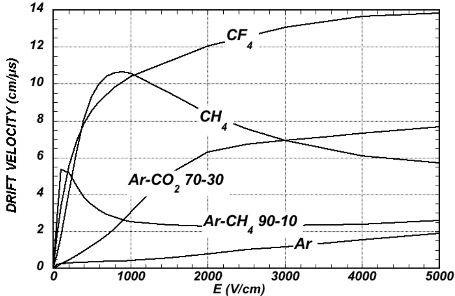
Figure 33.4: Computed electron drift velocity as a function of electric field in several gases at NTP and B = 0 [71].
