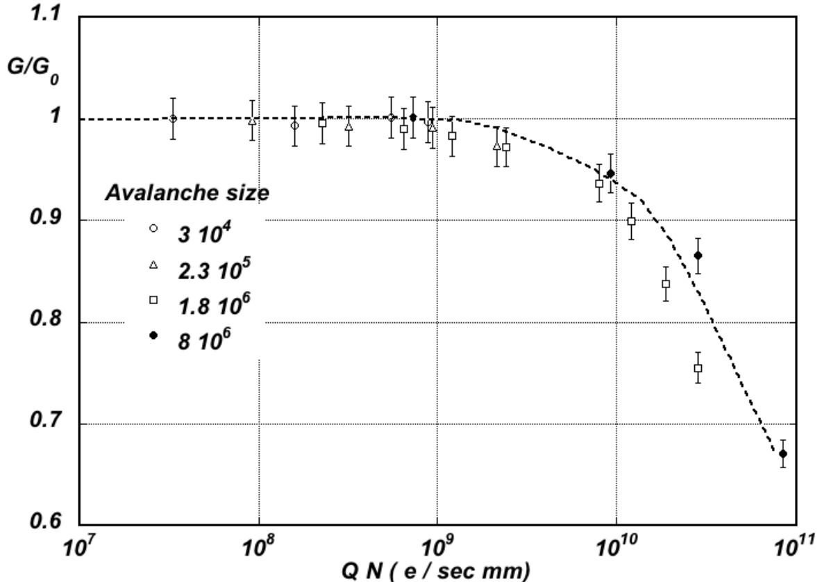
Figure 33.8: Charge rate dependence of normalized gas gain G/G_0 (relative to zero counting rate) in proportional thin-wire detectors [86]. Q is the total charge in single avalanche; N is the particle rate per wire length.
