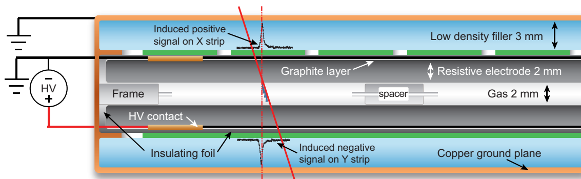
Figure 33.17: Schematic cross section of a generic single gap RPC.
