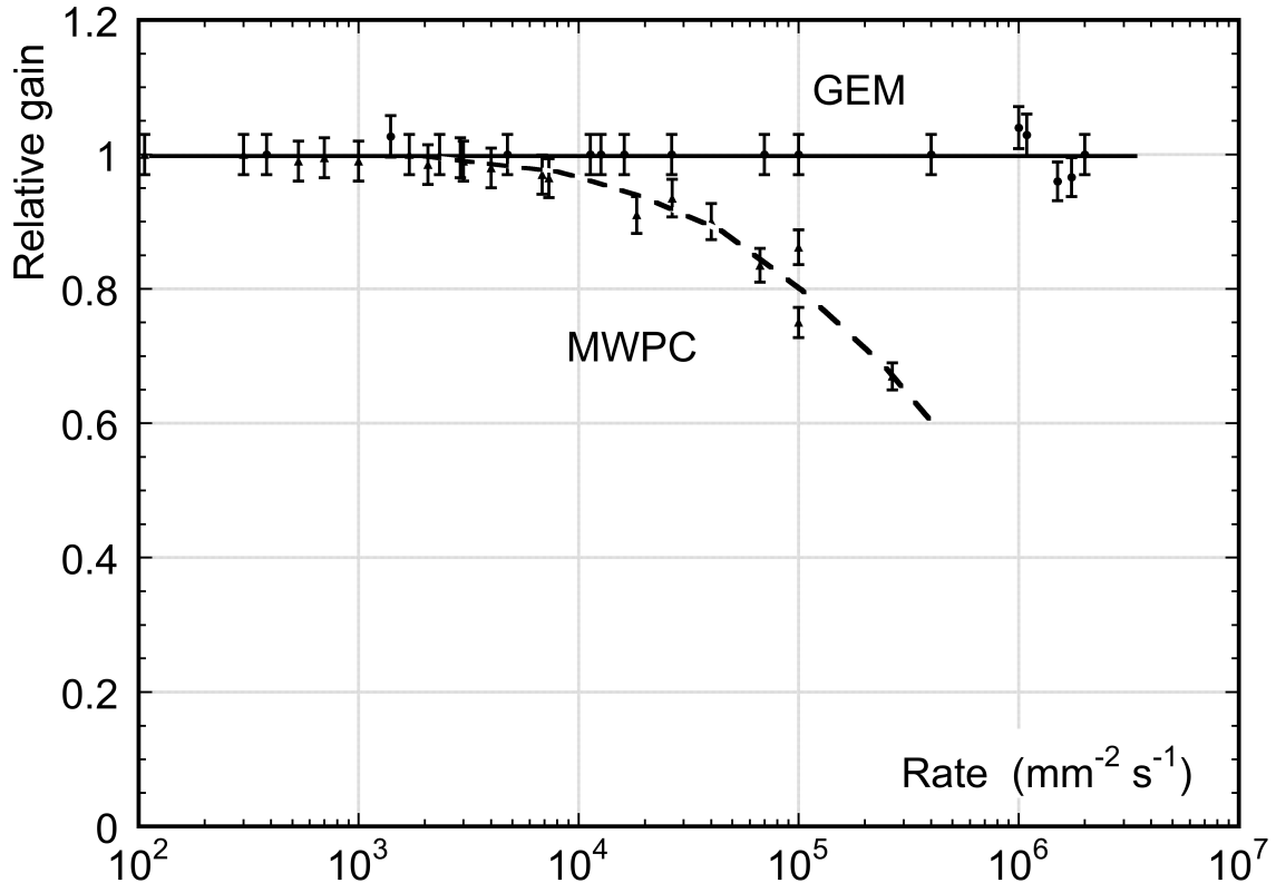
Figure 33.9: Normalized gas gain as a function of particle rate for MWPC [78] and GEM [92].
