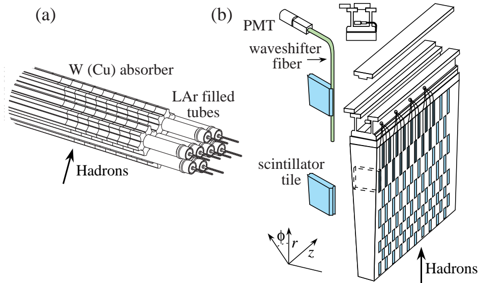
Figure 33.22: (a) ATLAS forward hadronic calorimeter structure (FCal2, 3) [158]. Tubes containing LAr are embedded in a mainly tungsten matrix. (b) ATLAS central calorimeter wedge; iron with plastic scintillator tile with wavelength-shifting fiber readout [159].
