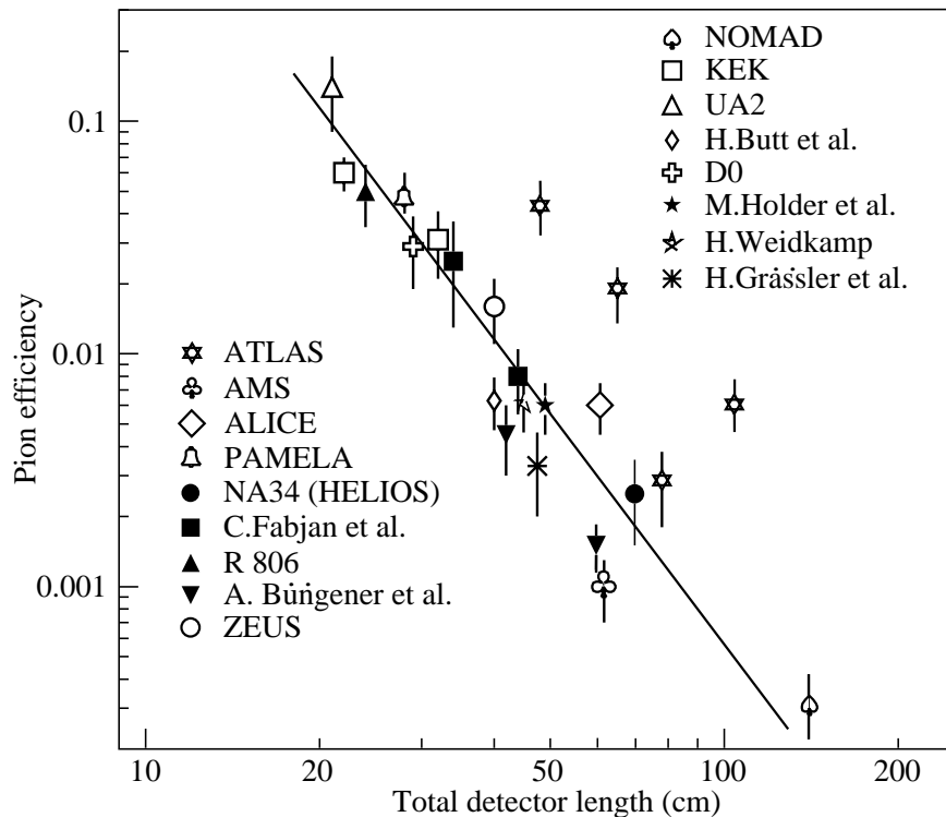
Figure 33.16: Pion efficiency measured (or predicted) for different TRDs as a function of the detector length for a fixed electron efficiency of 90%. The plot is taken from [112]. Results from more recent detectors are added from [113] and [114].
